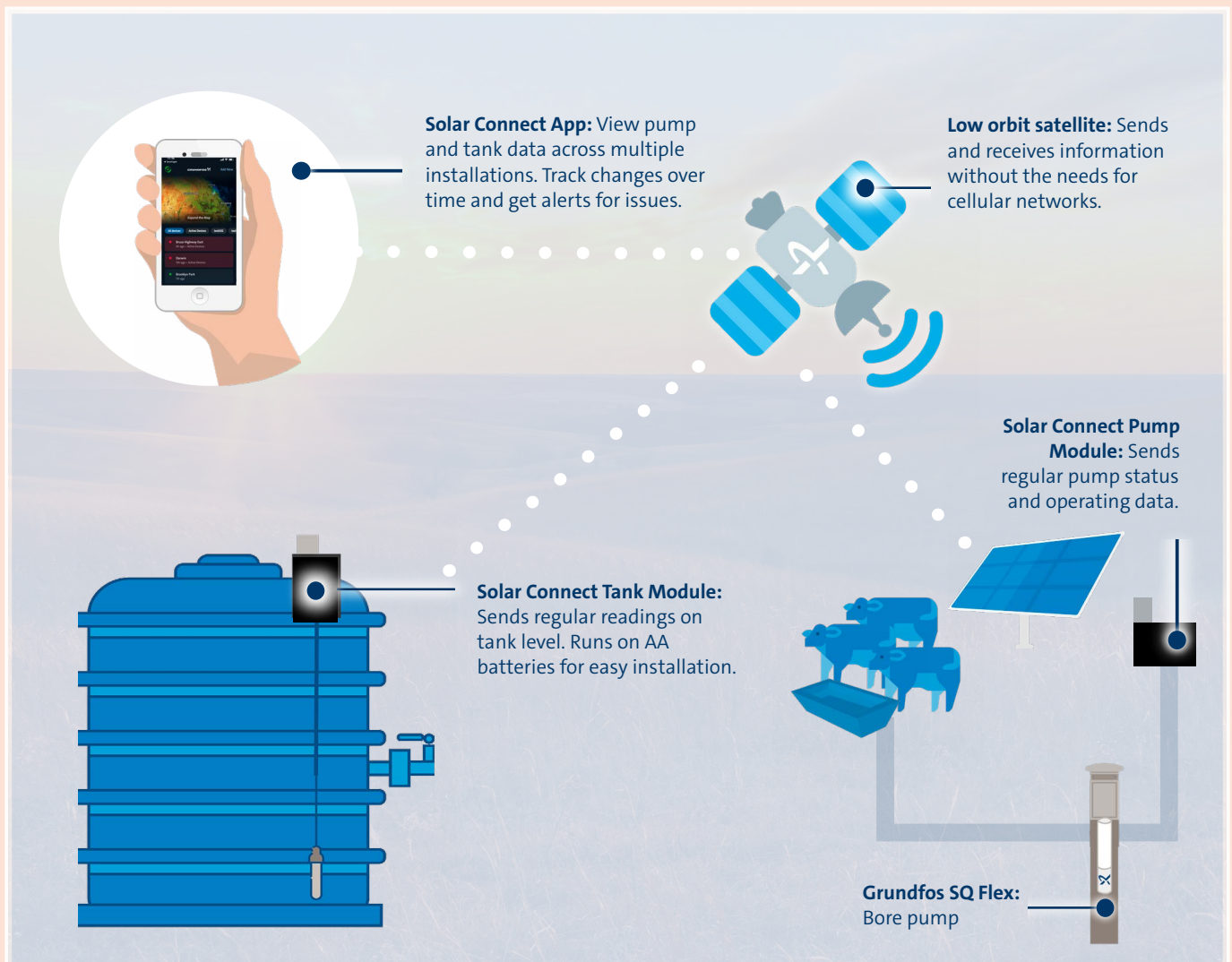
A typical Grundfos Solar Connect installation
